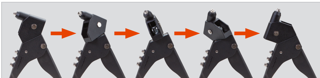
360° swivel head allows the user to set rivets at right angle or straight-on with a simple twist of rivet head
